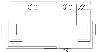
Installed using angle and pop rivets outside and inside
