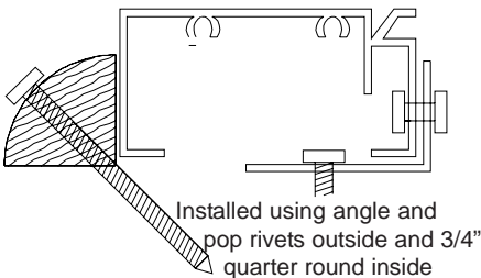
Installed using angle and pop rivets outside and inside
