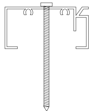
Installed using 2-1/2" hex head screws
