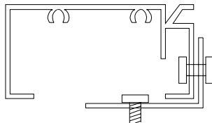
Installed using angle and pop rivets outside only
