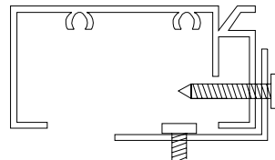
Installed using angle and 3/4" screws outside only
