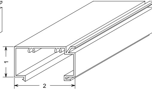
1" x 2" Interlock Frame
